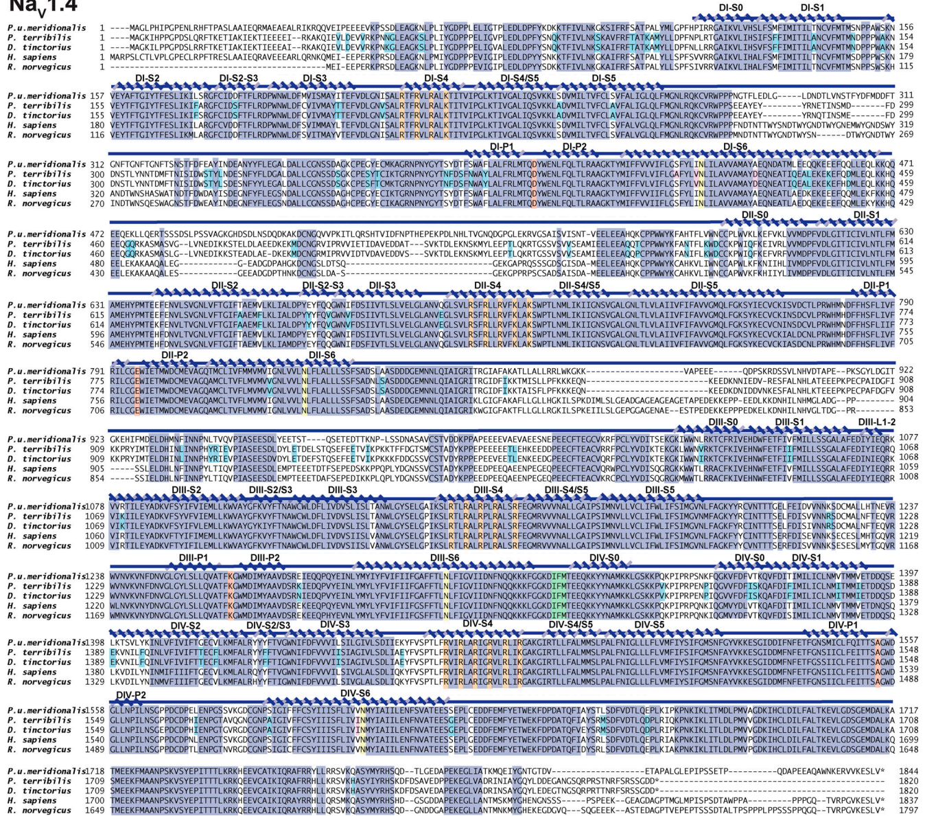
Figure S1. Pitohui and poison frog Na v 1.4 sequences. Sequence alignment of Pum Na v 1.4, Pt Na v 1.4, Dt Na v 1.4, Hs Na v 1.4 (RefSeq accession no. NP_000325.4), and Rn Na v 1.4 (RefSeq accession no. NP_037310.1). Key Na v features are highlighted as follows: selectivity filter DEKA (red), IFM peptide (green), conserved S6 Asn (yellow), S4 voltage sensor arginines (orange), poison frog variants (cyan), and sites highlighted by Tarvin et al. (2016; magenta) are indicated. Conserved residues are highlighted in dark blue. Secondary structure elements were labeled using boundaries from Yan et al. (2017).
