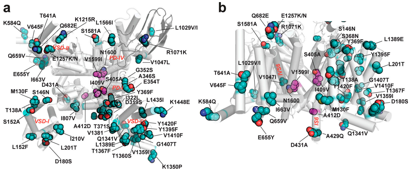
Figure 2. Structural context for poison frog Na v amino acid changes. (a and b) Locations of poison frog Na v amino acid variants reported here (cyan) and shared with Tarvin et al. (2016) (magenta). Variants are denoted human residue:residue number:frog variant using Pt Na v 1.4 numbering from Fig. S1. Residues are mapped on human Na v 1.4 (Protein Data Bank accession no. 6ADF; Pan et al., 2018). Na v 1.4 (white).
