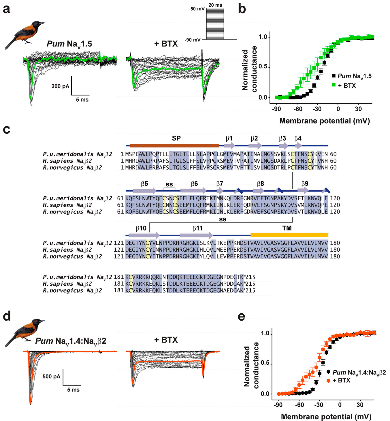
Figure S3. Pitohui Nav v 1.5 and Nav v 1.4:Nav v β2 complexes are BTX sensitive. (a) Exemplar current recordings for Pum Nav v 1.5 expressed in HEK293 cells in the absence (left) or presence (right) of 10 μM BTX. Trace at 0 mV is highlighted in each panel. Currents were evoked with the shown multistep depolarization protocol (inset). (b) G-V relationships in the absence (black squares) or presence (green squares) of 10 μM BTX. (c) Sequence alignment of Nav v β2 from Pum , Hs (RefSeq accession no. NP_004579.1), and Rn (RefSeq accession no. NP_037009.1). Signal peptide (SP), secondary structural elements from Das et al. (2016), conserved disulfide bond (ss), and transmembrane domain (TM) are indicated. (d) Exemplar current recordings for Pum Nav v 1.4:Nav v β2 expressed in HEK293 cells in the absence (left) or presence (right) of 10 μM BTX. Trace at 0 mV is highlighted in each panel. Currents were evoked with the shown multistep depolarization protocol (inset in a). (e) G-V relationships in the absence (black hexagons) or presence (red hexagons) of 10 μM BTX.
