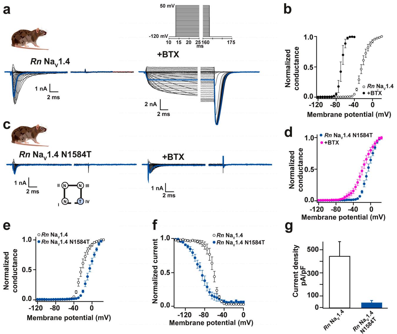
Figure S5. Functional costs of DIV-S6 Asn mutation in Rn Nav v 1.4 . (a and c) Exemplar current recordings for Rn Nav v 1.4 (a) and Rn Nav v 1.4 N1584T (c) expressed in CHO cells in the absence (left) or presence (right) of 10 \mu M BTX. Trace at 0 mV is highlighted in each panel. Currents were evoked with the shown multistep depolarization protocol (inset in a). (b and d) G-V relationships in the presence or absence of 10 \mu M BTX, Rn Nav v 1.4 (open circles), +BTX (black circles; b); and Rn Nav v 1.4 N1584T (blue circles), +BTX (magenta circles; d). (e) G-V relationships. (f) Steady-state inactivation voltage dependencies for Rn Nav v 1.4 (open circles) and Rn Nav v 1.4 N1584T (blue circles). (g) Current densities for Rn Nav v 1.4 (white) and Rn Nav v 1.4 N1584T (blue).
