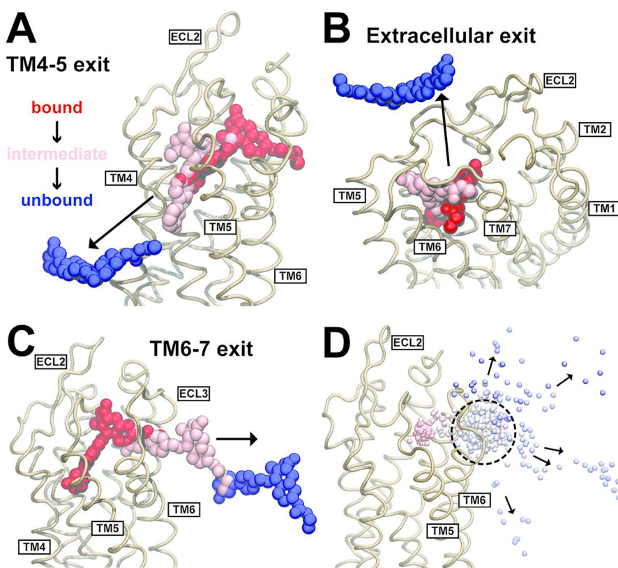
Figure 2. Ligand dissociation trajectories observed in TAMD simulations of vorapaxar dissociating from PAR1. (A) Ligand dissociation pathway between TM4 and TM5, observed in three simulations. (B) Ligand dissociation pathway into the extracellular solvent, observed in five simulations. (C) Ligand dissociation pathway between TM6 and TM7, observed in five simulations. In panels A–C, the PAR1 backbone is shown as light brown ribbons and vorapaxar atoms are shown as spheres. The crystallographic pose of vorapaxar is colored red, as well as representative poses from intermediate (pink) and unbound states (blue) observed in the simulations. (D) Overlay of the COM of vorapaxar (small spheres) during dissociation from PAR1 (light brown ribbons) between TM6 and TM7 in five different simulations. Simulation time progresses from red to white to blue in each simulation, and the time step is 180 ps. The metastable state is indicated by a dashed circle. The direction of vorapaxar motion is indicated by arrows.
