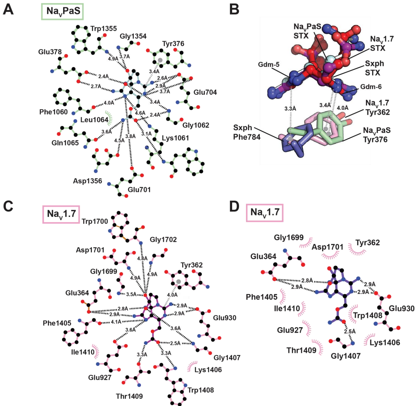
Fig. S8. Na v PaS:STX and Na v 1.7:STX interactions. (A) Na v PaS:STX interactions (PDB 6a91)(29) determined with LIGPLOT (67) and a cutoff of 5.0 Å. (B) Comparison of STX cation- \pi interactions with Sxph (blue), Na v PaS (green), and Na v 1.7 (magenta). STX from the Sxph:STX complex (red), Na v PaS:STX complex (cyan), and Na v 1.7:STX complex (violet) are indicated. (C and D) Na v 1.7:STX
